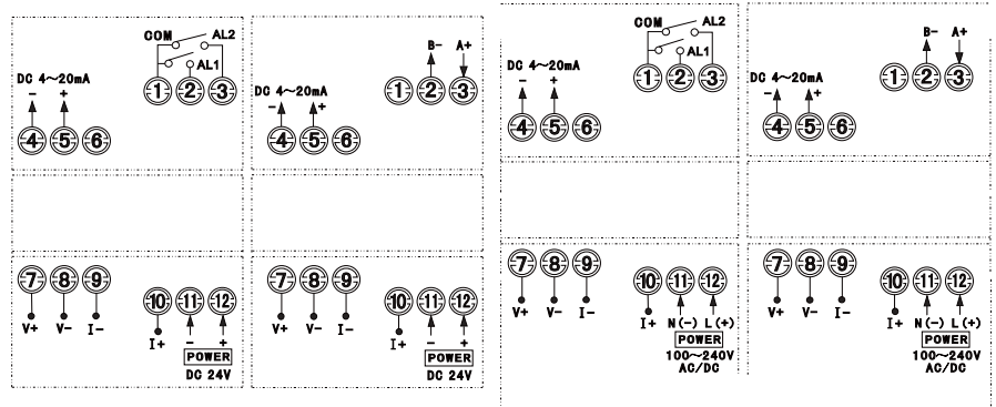
100-240V AC/DC power supply
